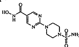
compound 3
